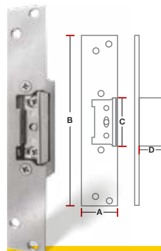
MEDIDAS EN mm. / MEASURES IN mm.
