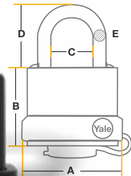
MEDIDAS EN mm. / MEASURES IN mm.
